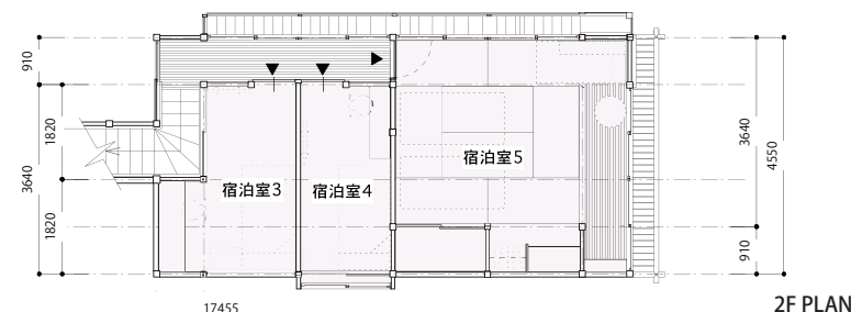
2F PLAN
