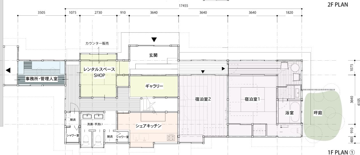
1F PLAN ①
